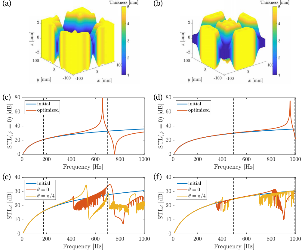
Figure 1: Obtained plate thickness profiles for single-leaf panel considering optimization regions of (a) a two-octave range centred at 350 Hz and (b) a one-octave range centred at 700 Hz. (c) STL for normal incidence for profile (a). (d) Same for profile (b). (e) STL for diffuse incidence for profile (a). (f) Same for profile (b).
