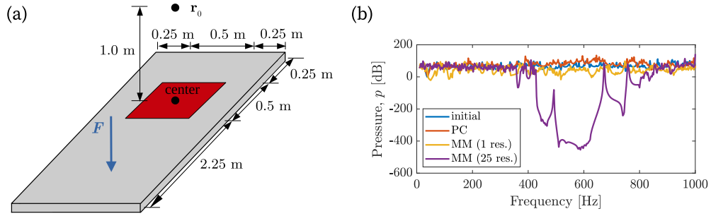
Figure 2: Numerical experiment to compare the effects of radiation. (a) The pressure at point \mathbf{r}_0 is computed considering the radiation of the red area for the simply supported plate, for a unit force applied at a distance of 2 m from its centre. (b) Pressure p at point \mathbf{r}_0 as a function of frequency.
