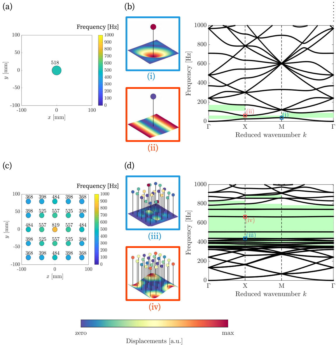
Figure 9: Optimisation results for the MM panel. (a) Single-resonator result with (b) dispersion diagram showing band gaps (green patches) and wave modes (i) and (ii) showing predominantly resonator (blue square) or plate displacements (red square). (c) Multiple-resonator result with (d) dispersion diagram showing several zero group velocity branches, opening large band gaps and wave modes (iii) and (iv).
