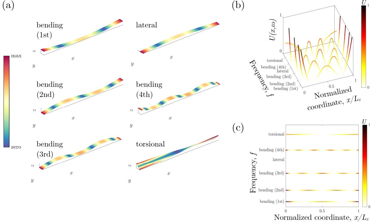
Figure S1: Representations of the tonotopic modal profile for a rectangular prism with dimension L_x \times L_y \times L_z ( L_x \gg L_y \gg L_z ). (a) The first 6 eigenmodes, with the color scale representing absolute values of displacements. (b) Tonotopic modal profile representation displaying the quadratic out-of-plane displacements mean. (c) Top views of the same plot in (b).
