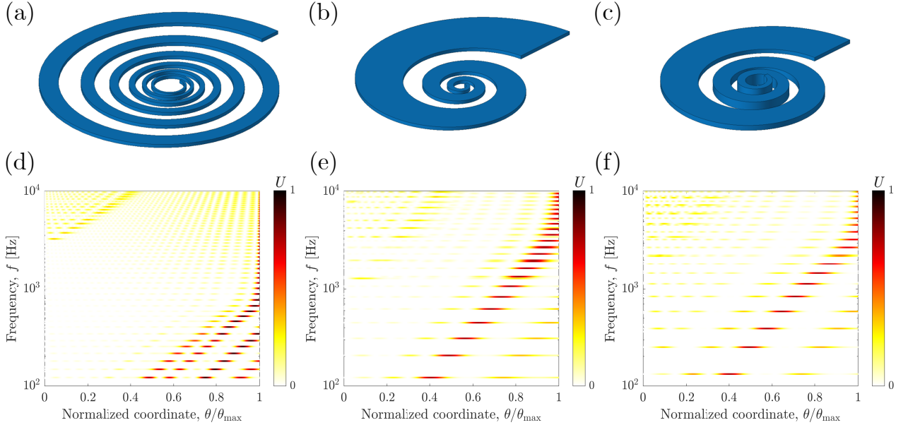
Figure S2: Structures obtained by increasing the (a) number of turns, (b) coiling, or (c) thickness increase of the baseline curved structure. (d) The smooth change in the structure cross section yielded by the increased number of turns hinders the isolation of peaks in the distribution of mean out-of-plane displacements. (e) Although limited by constraints for its physical construction, the increase in coiling facilitates the use of higher frequency modes. (f) Same observation as (e) for an increase in thickness.
