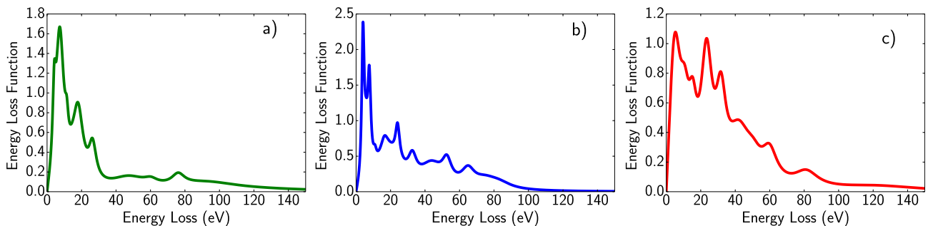
Fig. 9. Effective energy loss functions of Cu a), Ag b), and Au c) in the optical limit ( \vec{q} \rightarrow 0 ) obtained using Eq. (21). These ELFs were obtained by best-fitting the effective ELFs calculated by Nagatomi et al. [54].
