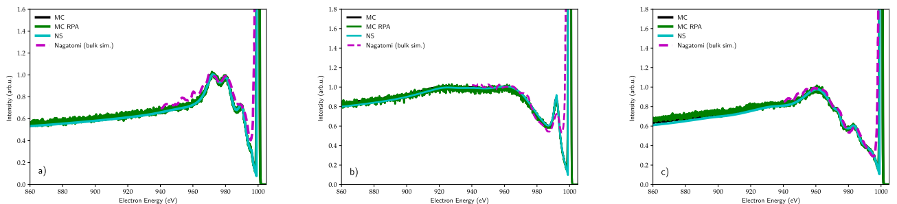
Fig. 11. REELS of a) Cu, b) Ag, and c) Au calculated using the full 3D bulk (RPA, green curve, see Eq. (25)) and high-limit (black curve, see Eq. (26)) dispersion laws in comparison to NS (cyan curve) and simulations by Nagatomi et al. (violet curve [54]).
