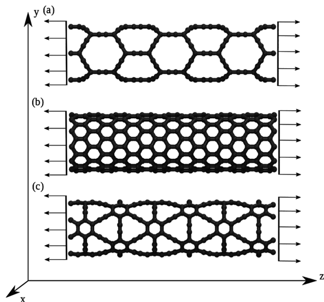
Fig. 2. Schematic of the tensile stress/strain simulations for: (a) \alpha -GNT; (b) CNT, and; (c) \gamma -GNT. The arrows indicate the stretching (axial) direction.
