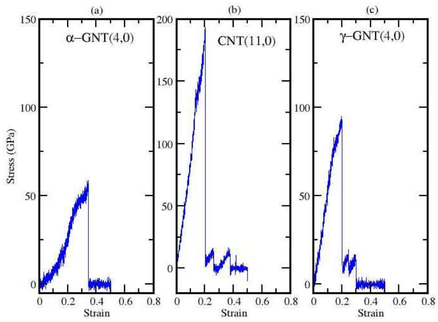
Figure 5. Stress strain curve of \alpha -GNT(4,0), CNT(11,0) and \gamma -GNT(4,0) using ReaxFF-FC [5] set of parameters.
