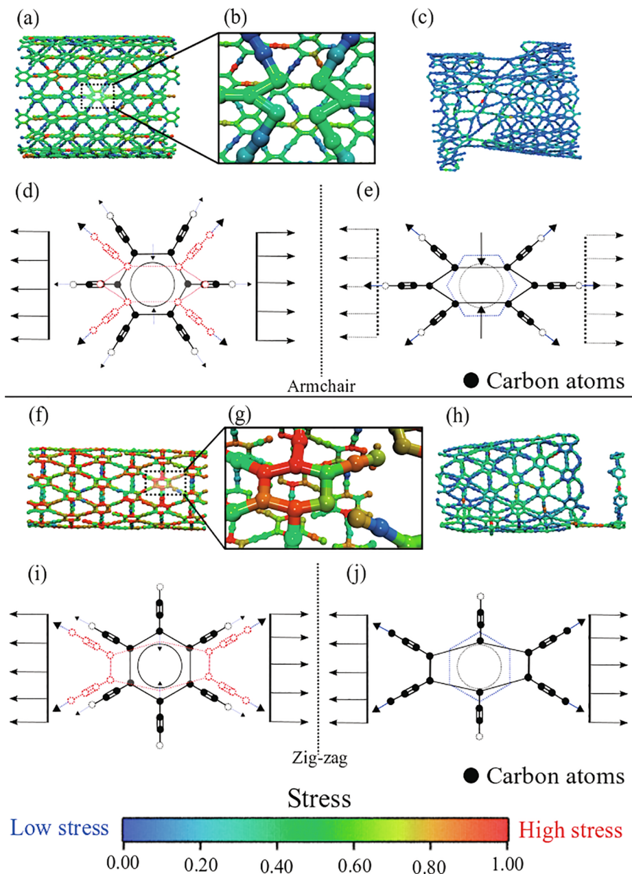
Fig. 4. Representative MD snapshots of a tensile stretch of the armchair (4, 4) (top) and zigzag (4, 0) (bottom) \gamma -GNT. (a, f) Lateral view of the strained nanotube colored accordingly to the von Mises stress values (low stress in blue and high stress in red). (b, g) Zoomed view of the starting of bond breaking. (c, h) MD snapshot of the nanotube just after fracture. Diagrams showing the ring dynamics of the armchair ((d) and (e)) and zigzag ((i) and (j)) \gamma -GNT can also be seen.
