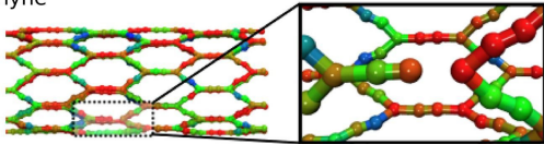
\alpha -Graphyne
