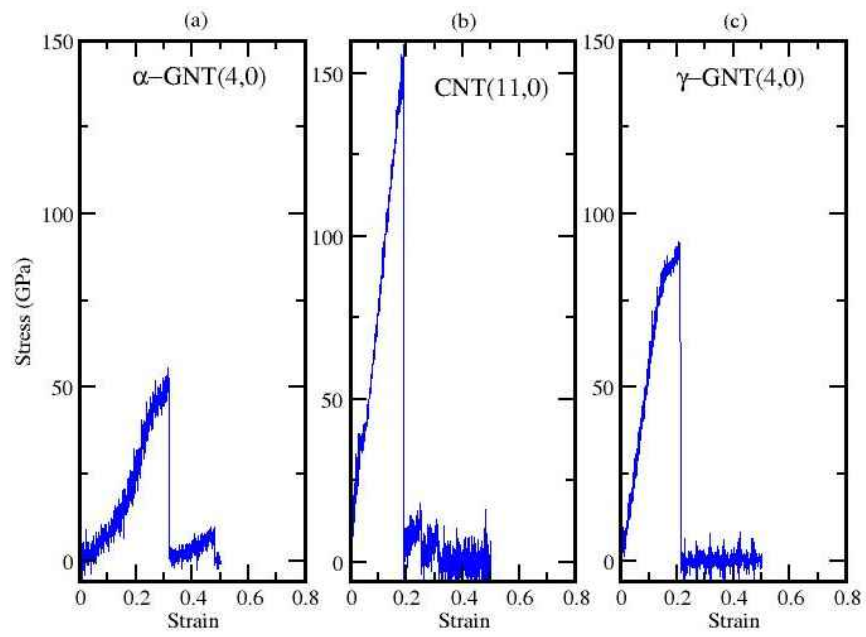
Figure 4. Stress strain curve of \alpha -GNT(4,0), CNT(11,0) and \gamma -GNT(4,0) using ReaxFF-Budzien [4] set of parameters.
