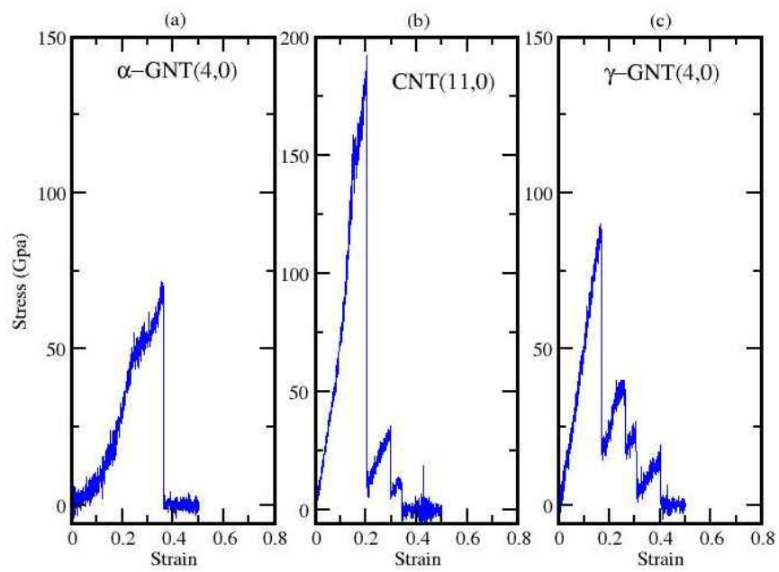
Figure 6. Stress strain curve of a-GNT(4,0), CNT(11,0) and g-GNT(4,0) using ReaxFF-FeOH [6] set of parameters.
