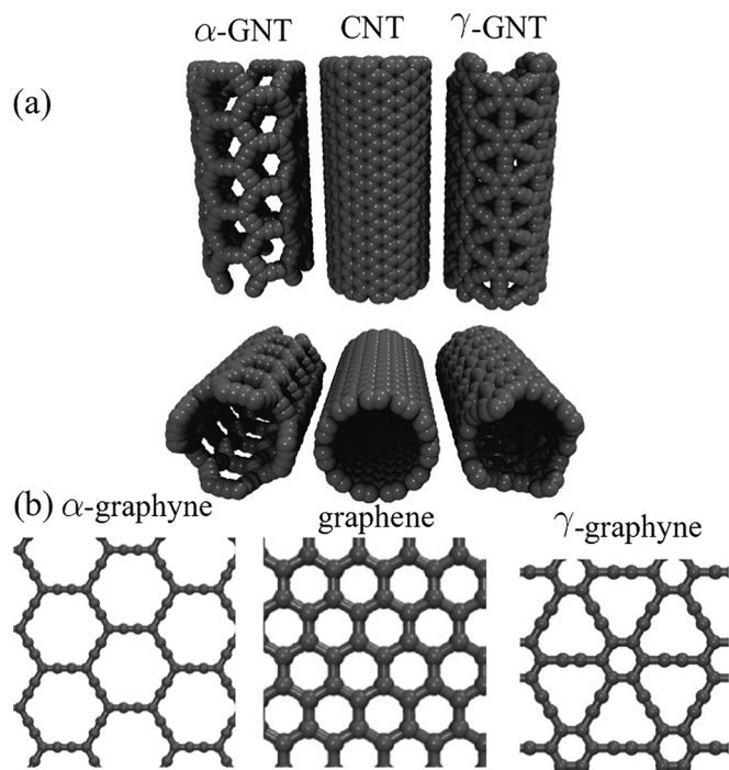
Fig. 1. (a) Quasi-1D nanotubes and (b) 2D carbon nanostructures. (a) From left to right: \alpha -GNT(4, 4), CNT(11, 11), and \gamma -GNT(4, 4). (b) 2D carbon sheets that generated the above nanotubes.
