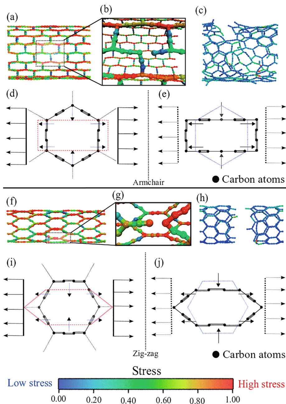
Fig. 3. Representative MD snapshots of a tensile stretch of the armchair (4, 0) (top) and zigzag (4, 0) (bottom) \alpha -GNT. (a, f) Lateral view of the strained nanotube colored accordingly to the von Mises stress values (low stress in blue and high stress in red). (b, g) Zoomed view of the starting of bond breaking. (c, h) MD snapshot of the nanotube just after fracture. Diagrams showing the ring dynamics of the armchair ((d) and (e)) and zigzag ((i) and (j)) \alpha -GNT can also be seen.
