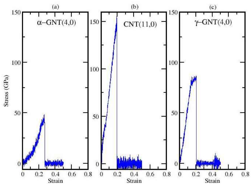
Figure 8. Stress strain curve of a-GNT(4,0), CNT(11,0) and g-GNT(4,0) ReaxFF-RDX [8] set of parameters.
