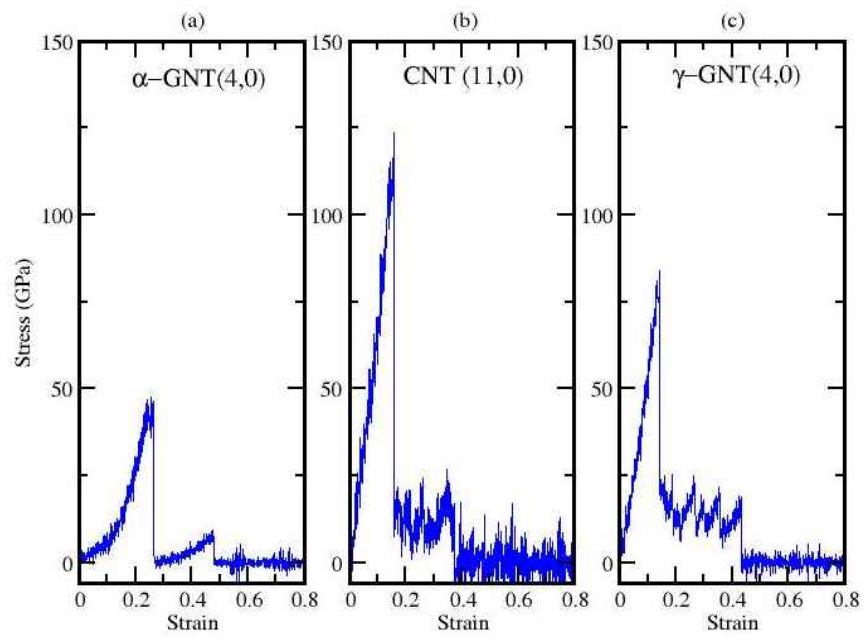
Figure 3. Stress strain curve of \alpha -GNT(4,0), CNT(11,0) and \gamma -GNT(4,0) using ReaxFF-Mattsson [3] set of parameters.
