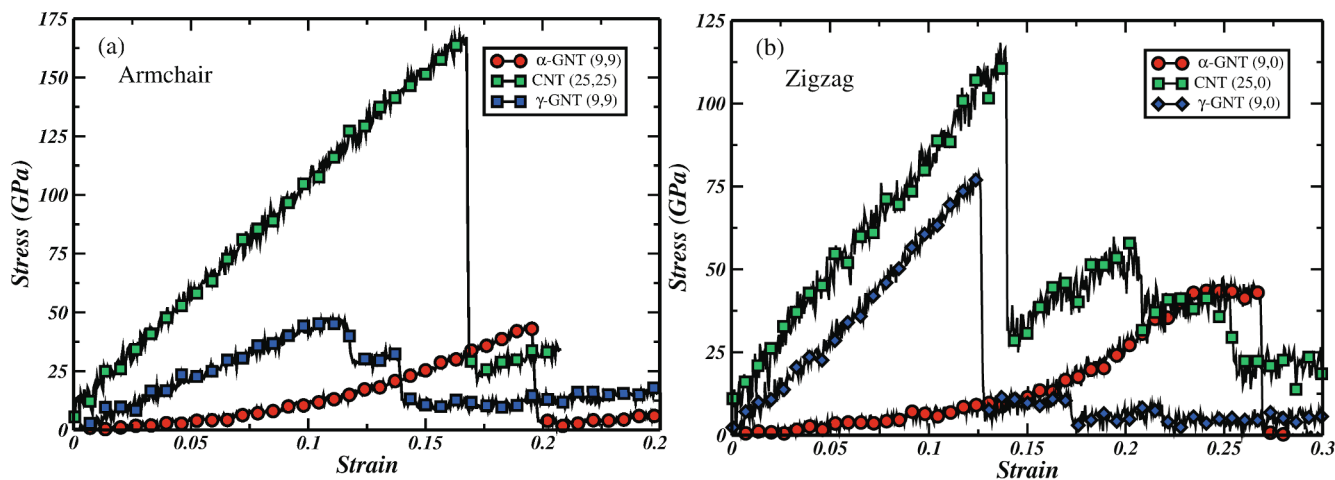
Fig. 6. Stress-strain curves obtained for CNTs ((25, 25) and (25, 0), green color), \alpha -GNTs ((9, 9) and (9, 0), red color), and \gamma -GNTs ((9, 9) and (9, 0), blue color) at 300 K.
