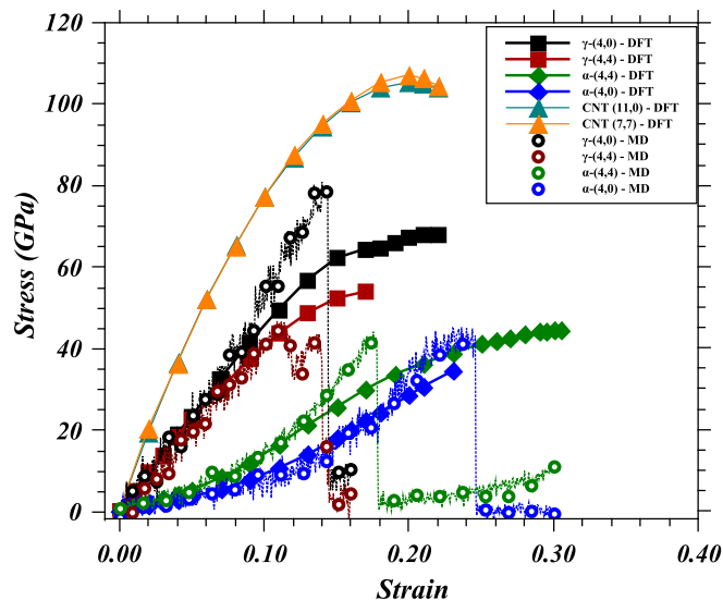
Fig. 7. Stress-strain curves obtained from DFT and MD calculations for conventional CNTs, \alpha -GNTs and \gamma -GNTs.
