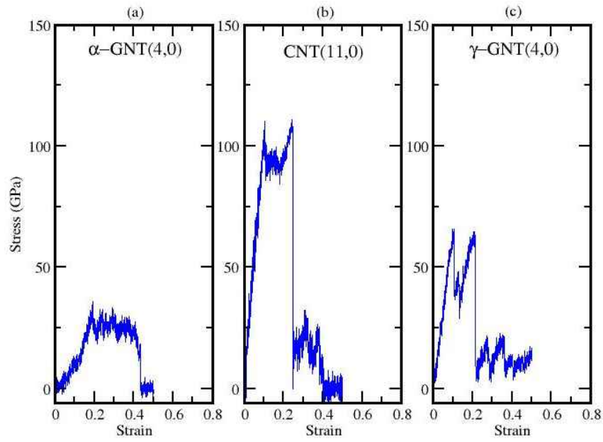
Figure 9. Stress strain curve of \alpha -GNT(4,0), CNT(11,0) and \gamma -GNT(4,0) using ReaxFF-VOCH [9] set of parameters.
