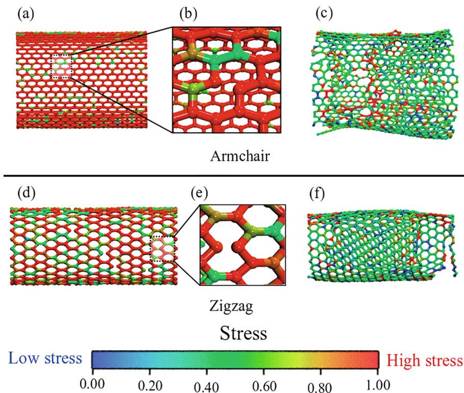
Fig. 5. Representative MD snapshots of a tensile stretch of conventional CNTs (armchair (11, 11) (top) and zigzag (11, 0) (bottom)). (a, d) Lateral view of the strained nanotube colored accordingly to the von Mises stress values (low stress in blue and high stress in red). (b, e) Zoomed view of the starting of bond breaking. (c, f) MD snapshot of the nanotube just after fracture.
