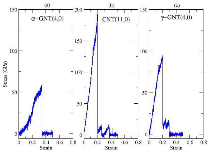
Figure 7. Stress strain curve of \alpha -GNT(4,0), CNT(11,0) and \gamma -GNT(4,0) using ReaxFF-Muller [7] set of parameters.
