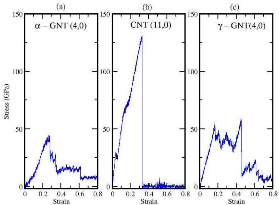
Figure 1. Stress strain curve of a-GNT(4,0), CNT(11,0) and g-GNT(4,0) using ReaxFF-2013 [1] parameters.
