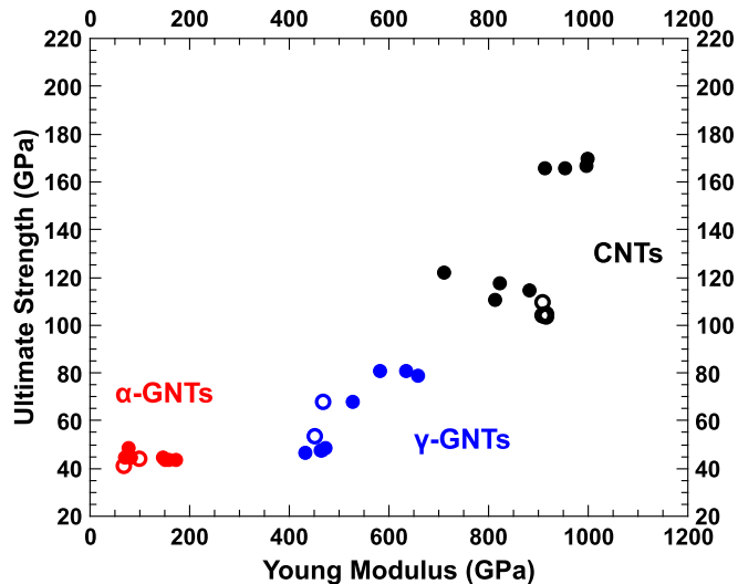
Fig. 8. Ultimate Strength (US) values as function of the Young's modulus values for different structures. CNTs, \gamma -GNTs and \alpha -GNTs are respectively in black, blue and red. Filled (open) symbols hold for MD (DFT) results.
