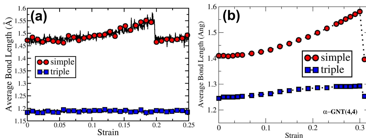
Figure 10: Average bond length evolution of simple and triple bonds in \alpha -GNT(9,9) nanotubes within MD framework (a) and \alpha -GNT(4,4) within DFT framework (b).
