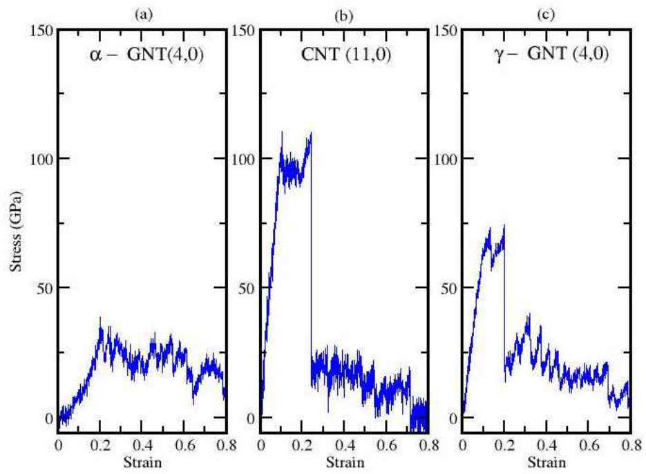
Figure 2. Stress strain curve of \alpha -GNT(4,0), CNT(11,0) and \gamma -GNT(4,0) using ReaxFF-CHO [2] parameters.
