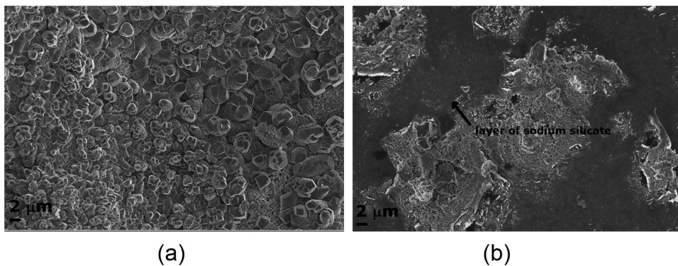
Figure 8. FE-SEM micrographs. (a) Inner surface of the extruded hollow tube without coating: the microstructure of the tube is clearly visible. (b) Inner surface of the hollow tube coated with the sodium silicate: the microstructure of the tube is covered by a homogeneous layer of coating.
