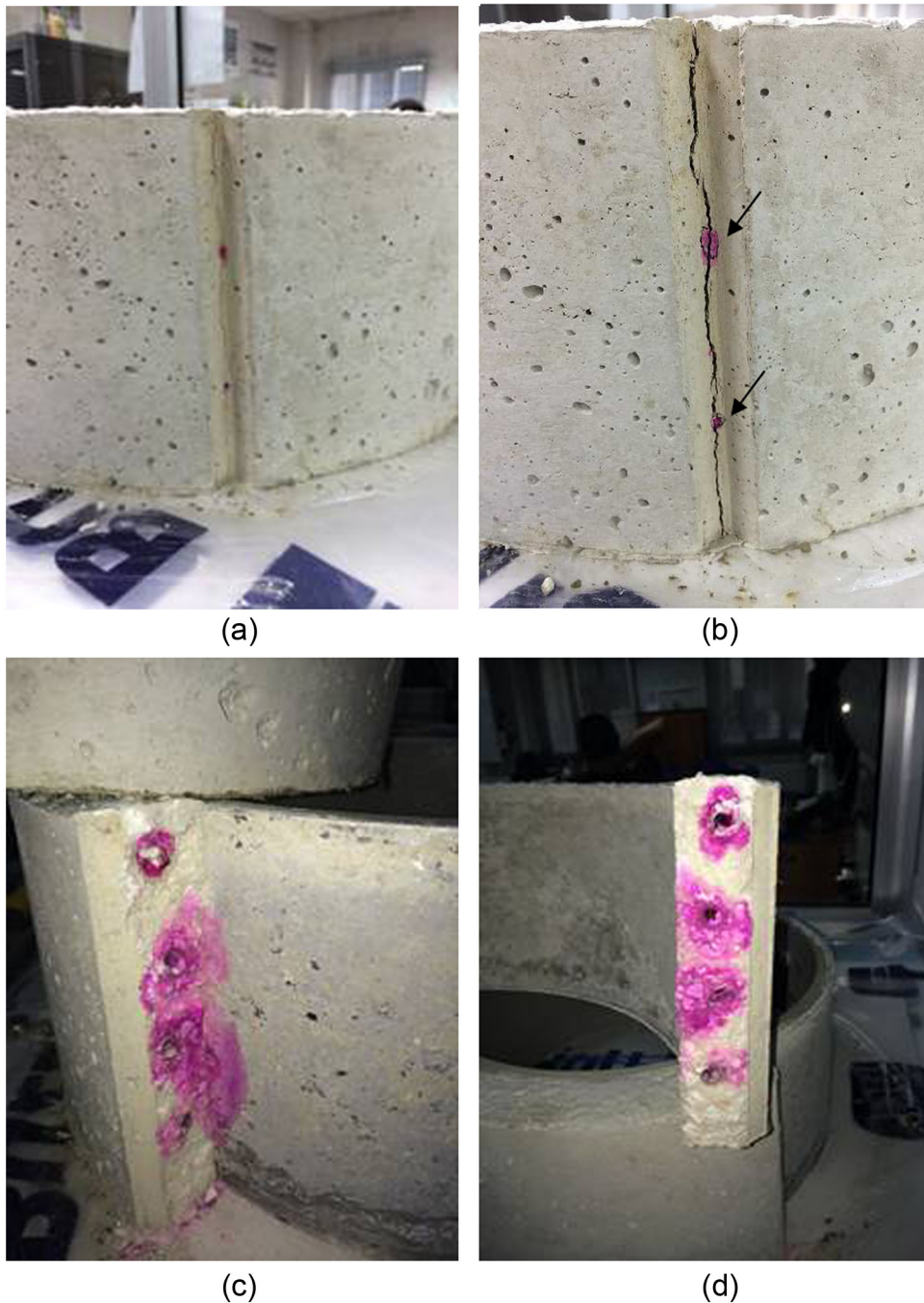
Figure 2. Ring tests images: (a) first micro-cracking leading to the diffusion of Rhodamine B water solution up to the external surface of the concrete annular specimen; (b) macro-cracking; (c) and (d) crack surfaces with Rhodamine-colored water diffusion around the hollow tubes.
