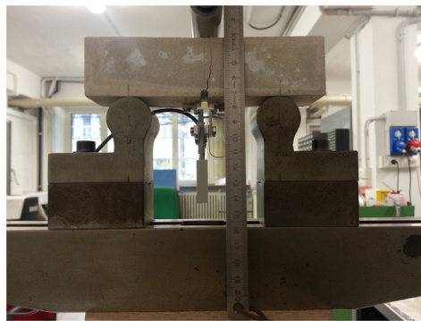
Figure 6. Specimen under load during the pre-loading stage with maximum CMOD of approximately 800 \mu\text{m} .
