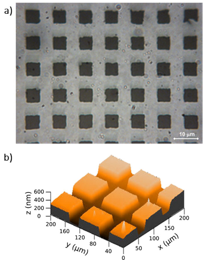
Fig. 1. a) Optical microscope image of a diamond sample after irradiation with a 40 MeV Br beam at a fluence of 5 \times 10^{13} cm -2 . An 11 μm mesh mask with 5.5 μm square apertures was used for irradiation. Dark areas of 5.5 \times 5.5 μm 2 correspond to the irradiated sample surface, whereas the surrounding grey area corresponds to the unirradiated surface (i.e. the mask-covered regions). b) Surface topography, as measured with a profilometer, of a single-crystal diamond sample after irradiation with a 10 MeV Au beam at a fluence of 5 \times 10^{14} cm -2 . An 80 μm mesh mask with 60 μm square apertures was used for the irradiation.
