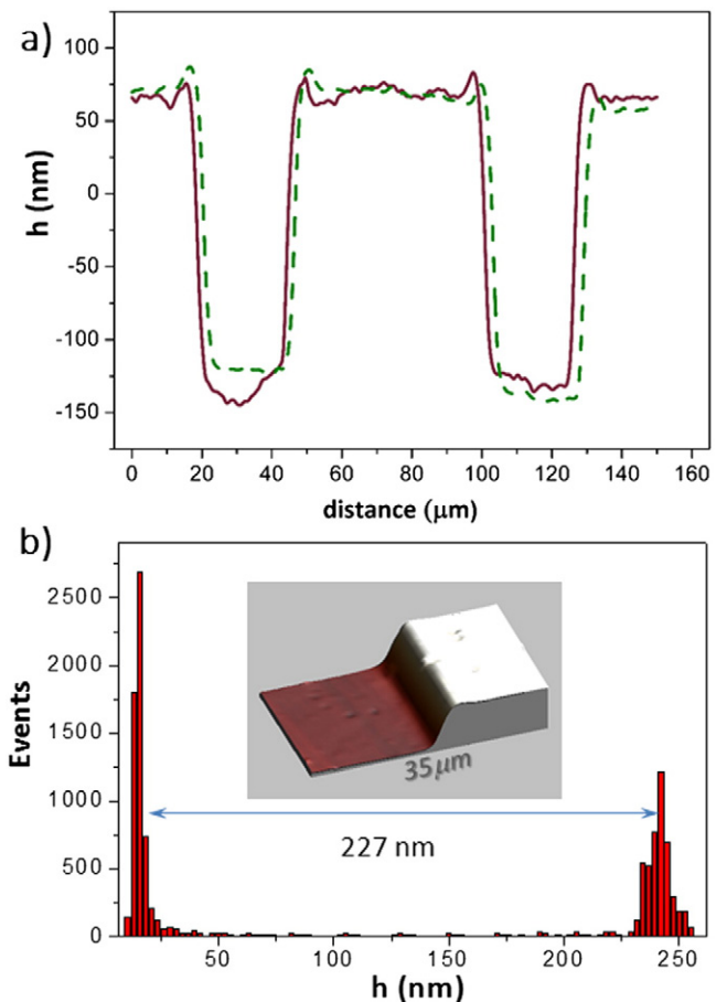
Fig. 3. a) Line scans taken at two representative points of a 2D profilometry scan, yielding an average height \Delta h = 204 \text{ nm} . b) Height analysis. A 3D image corresponding to a selected area containing part of one structure and part of the canyon is selected to illustrate the procedure. The histogram represents the frequency (events) of each height value on the image. It shows two main peaks. The peak at the left corresponds to the base of the canyon and that at the right to the plateau. The difference in height or step height is therefore the distance between the two peak centers, i.e. \Delta h = 227 \text{ nm} in this case. Both graphs correspond to the same sample. Irradiation parameters are those given in Fig. 2.
