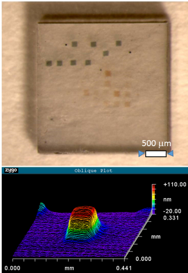
Fig. 4. Optical micrograph of a CVD diamond sample irradiated with 2 MeV H ions. Increasing implantation fluence corresponds to increasing area opacity (upper). Example of a measured swelling profile using white-light interferometry (lower).
